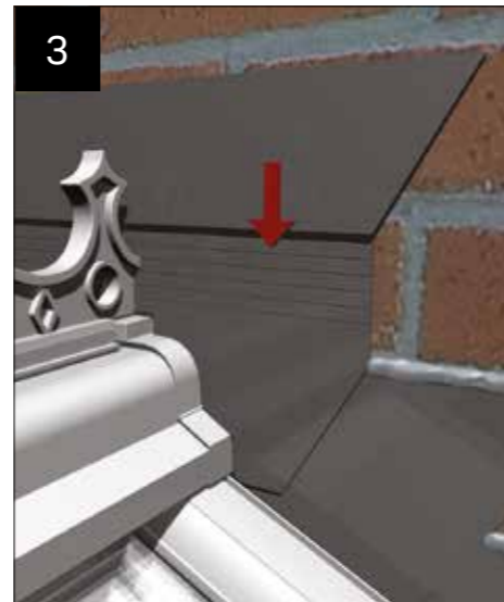
3 Offer up the horizontal flashing and cut ends as appropriate.
